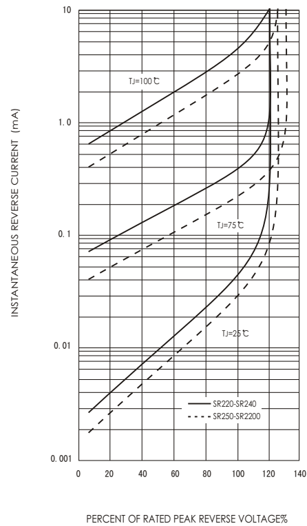
FIG.4-TYPICAL REVERSE CHARACTERISTICS
