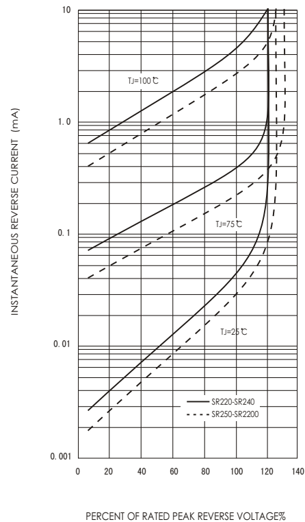
FIG.4-TYPICAL REVERSE CHARACTERISTICS
