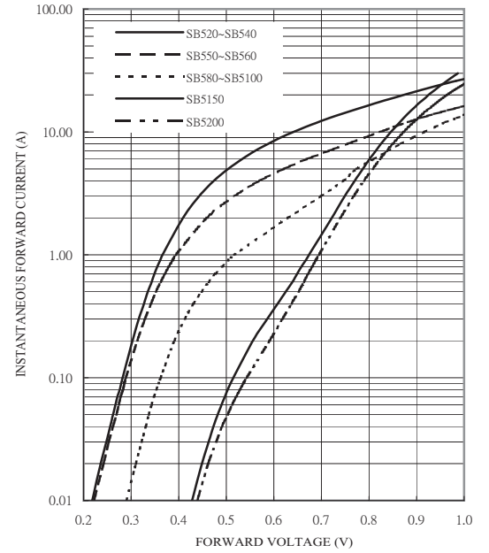
FIG. 2-TYPICAL FORWARD CHARACTERISTICS
