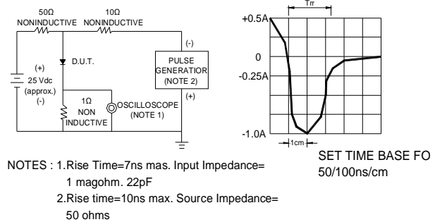
F1G.6-TEST CIRCUIT DIAGRAM AND REVERSE RECOVERY TIME CHARACTERISTIC
