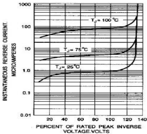
Fig. 3-TYPICAL REVERSE CHARACTERISTICS
