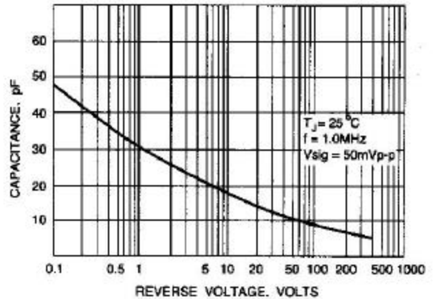
Fig. 6-TYPICAL JUNCTION CAPACITANCE
