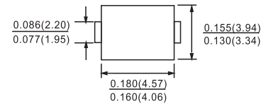
DO-214AA(SMB)
