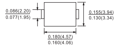
DO-214AA(SMB)
