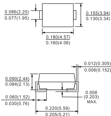
DO-214AA(SMB)
