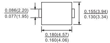
DO-214AA(SMB)
