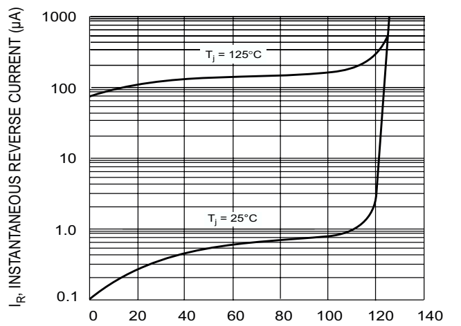
PERCENT OF RATED PEAK REVERSE VOLTAGE (%) Fig. 4 Typical Reverse Characteristics
