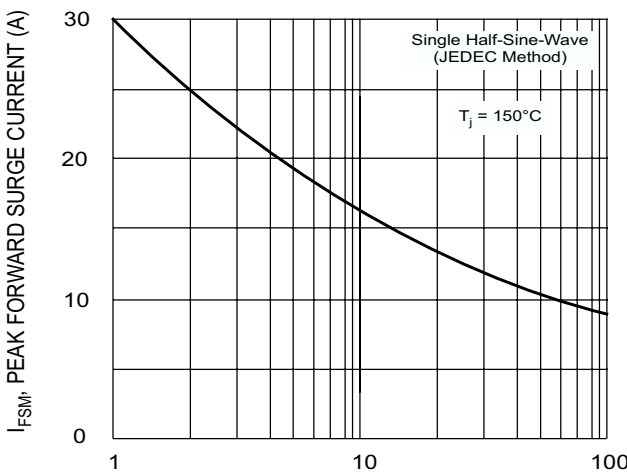
Fig. 3 Forward Surge Current Derating Curve
