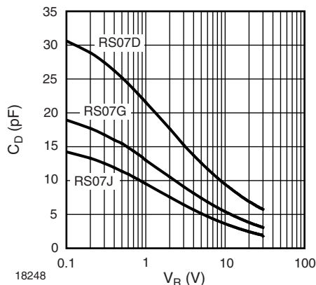
Figure 4. Typ. Diode Capacitance vs. Reverse Voltage
