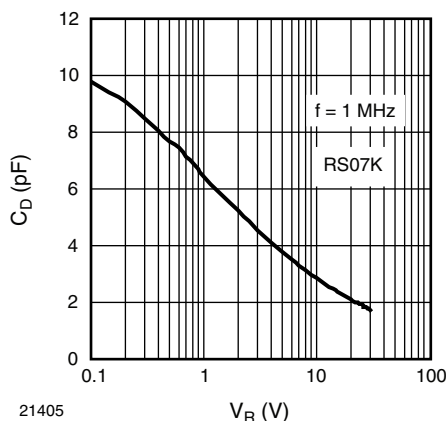
Figure 5. Typ. Diode Capacitance vs. Reverse Voltage
