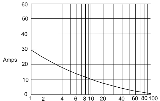
Figure 5 Peak Forward Surge Current
