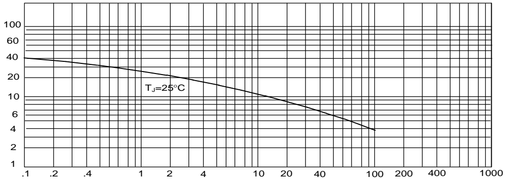
Figure 3 Junction Capacitance
