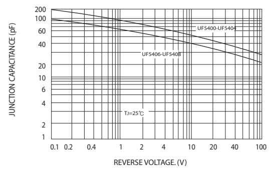
FIG6-TYPICAL JUNCTION CAPACITANCE
