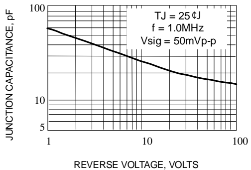
Fig. 6-TYPICAL JUNCTION CAPACITANCE
