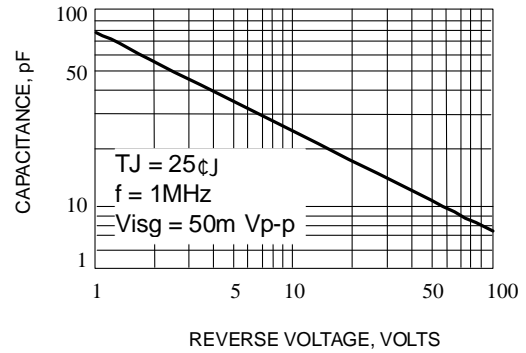
Fig. 4-TYPICAL JUNCTION CAPACITANCE
