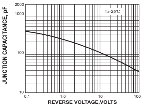
FIG. 5-TYPICAL JUNCTION CAPACITANCE
